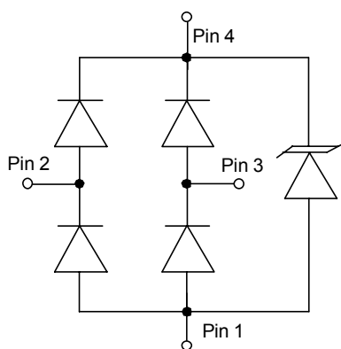
Circuit Diagram
